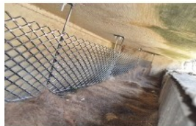
Inlet Guard with hair mat inside a storm drain
